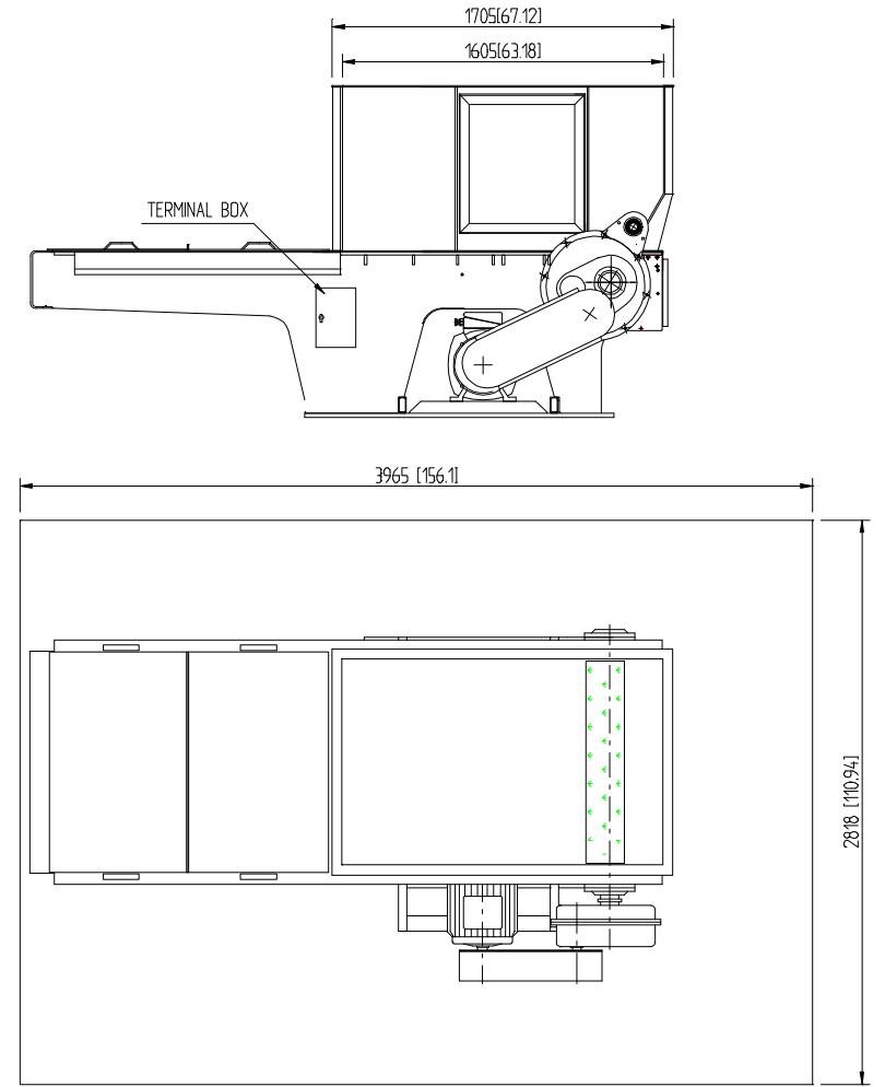
RECOMMENDED INSTALLATION DIMENSIONS
